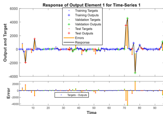
FIGURE 14. Response of Output Element for Residual Time-Series
