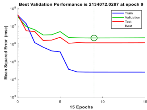
FIGURE 12. Training performance
