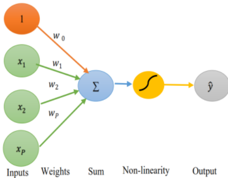
FIGURE 2. The Perceptron Forward Propagation
