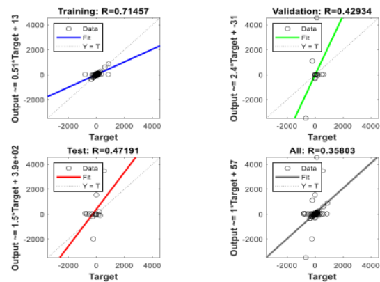
FIGURE 13. Model Summary
