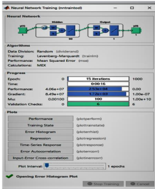
FIGURE 11. Trained output
