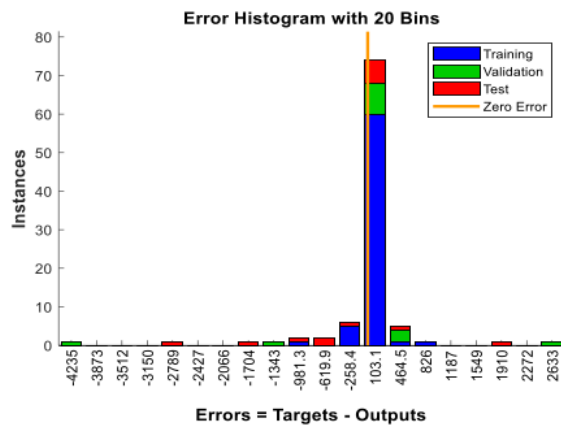
FIGURE 15. Errors of the fitted Residual neural network
