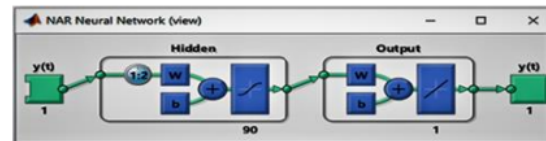
FIGURE 9. Closed loop NARNET architecture
