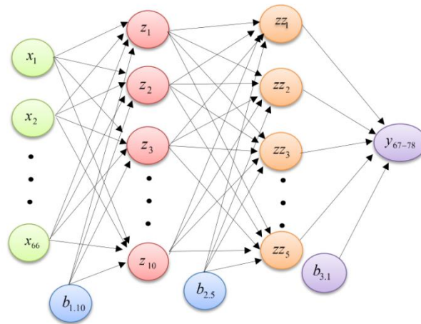
Figure 1. ANN Architecture for Data Prediction
