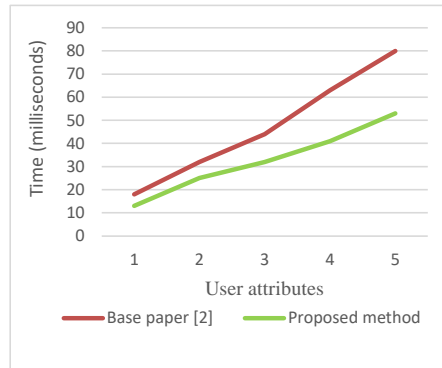
Figure 3 - Comparison of decoding costs in the proposed method and the basic paper
