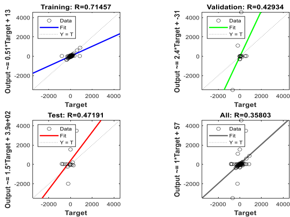
FIGURE 13. Model summary.
