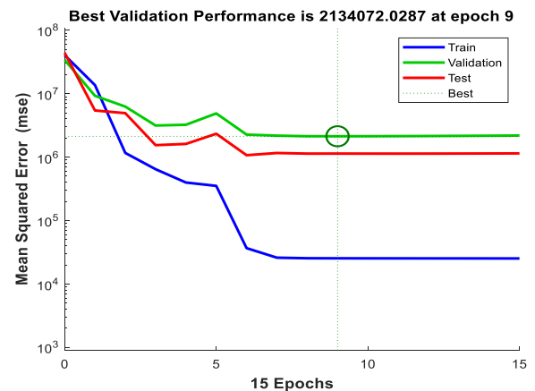
FIGURE 12. Training performance.
