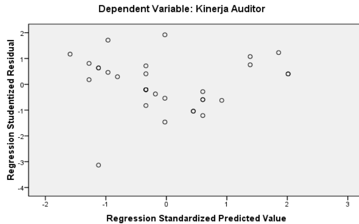
Scatterplot
