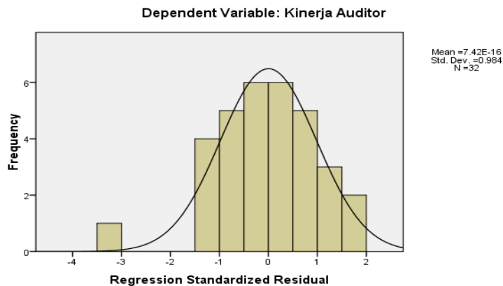
Histogram
