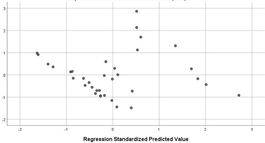
Scatterplot
