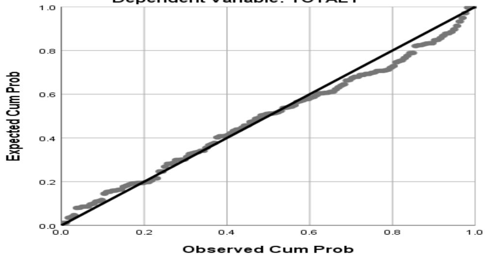
Normal P-P Plot of Regression Standardized Residual Dependent Variable: TOTALY
