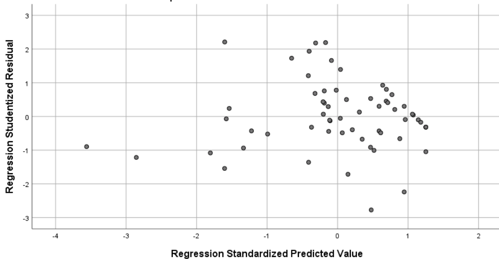
Scatterplot
