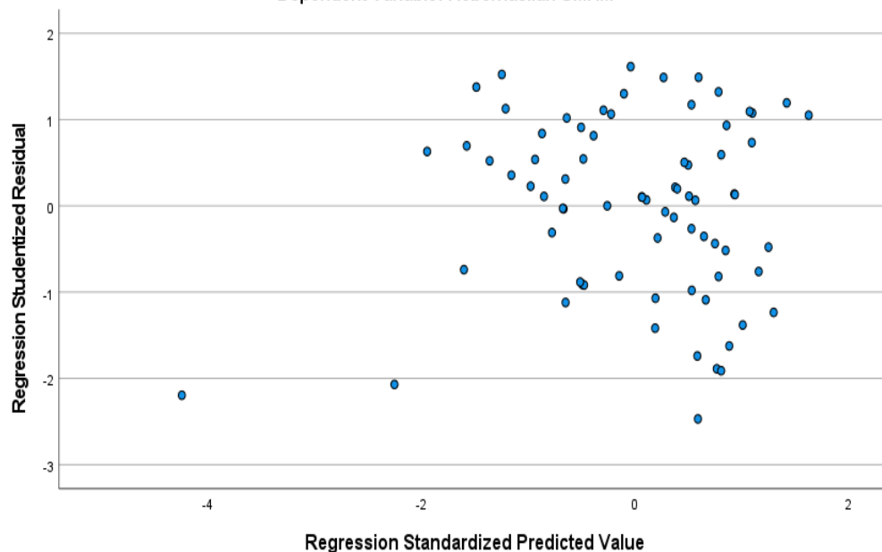
Scatterplot
