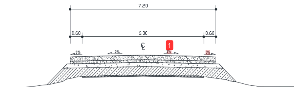
Gambar 4. 6 Typical Potongan Melintang (Sumber: Hasil analisa (2025))
