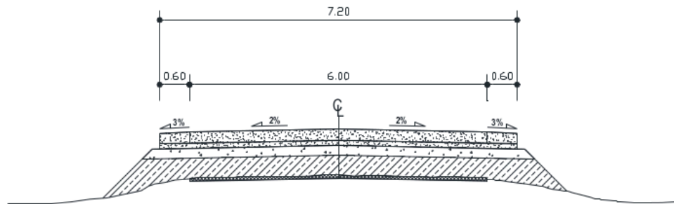
Gambar 4. 5 Typical Potongan Melintang (Sumber: Hasil analisa (2025))
