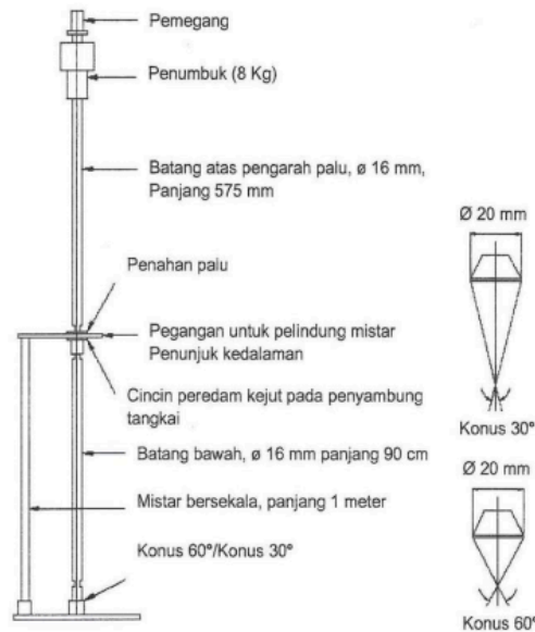
Gambar 2. 18 Alat Dynamic Cone Penetrometer (DCP)
