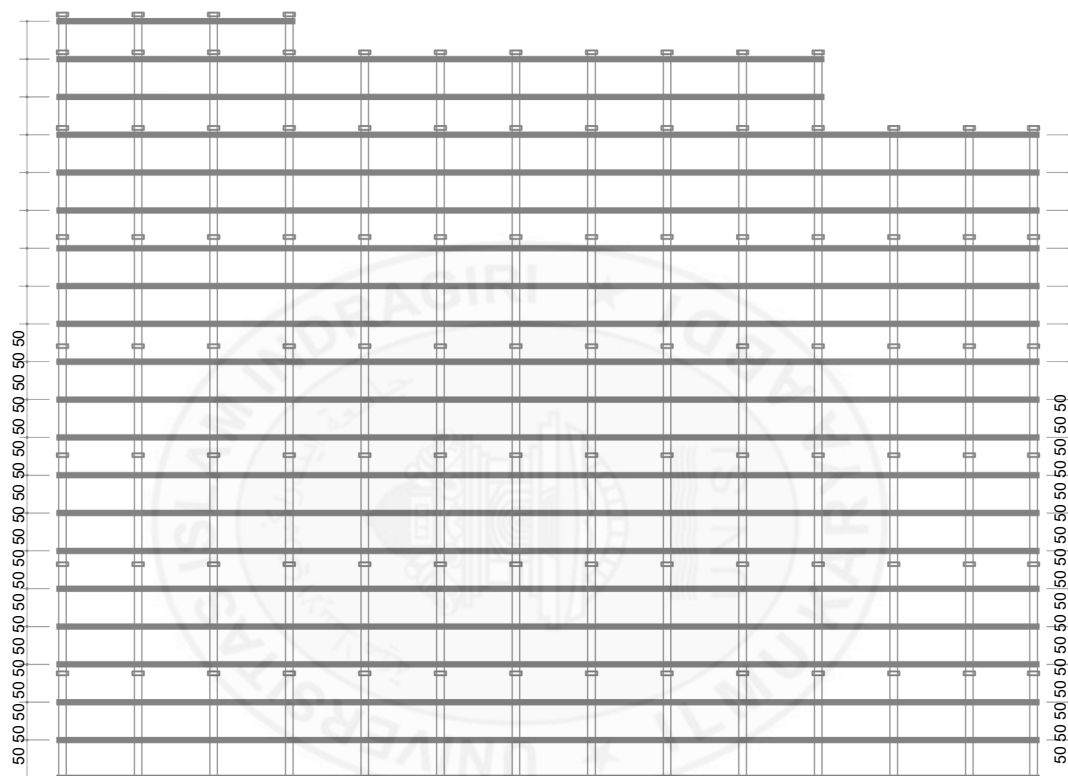
DENAH GELAGAR LANTAI
